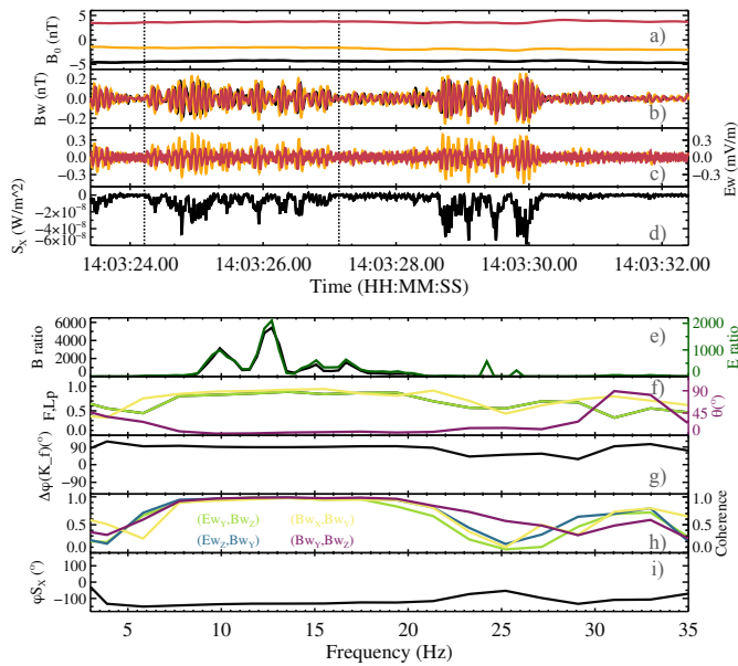
Fig. 1: Analysis of whistler waves detected by Solar Orbiter RPW on 2020 July, 22nd around 14:03. Panels a) to d) : The X component is in black, Y is in red, and Z is in yellow (spacecraft reference frame). Panel a) : Background magnetic field B_0 . Panels b) and c) : Waveforms of the magnetic B_w and electric E_w fields. Panel d) : X component of the Poynting vector ( S_X ). For Panels c) and d) we used an effective length of the electric antennas equal to 6 m. Panels e) to i) : Analysis of the wave packet delimited by vertical dotted lines. Panel e) : Ratio of the magnetic power spectrum to the median power spectrum of the day (black) and the same for the electric field (green, with the Y and Z components only). Panel f) : Polarization (Lp in orange), planarity (F in black), and propagation angle ( \theta in purple). Panel g) : Phase shift between B_{w_x} and B_{w_y} (in the wave reference frame with \mathbf{k} = k_z , see Section 2.1). Panel h) : Spectral coherence between different components. Panel i) : Phase of the X component of the Poynting vector \varphi_{S_X} .
