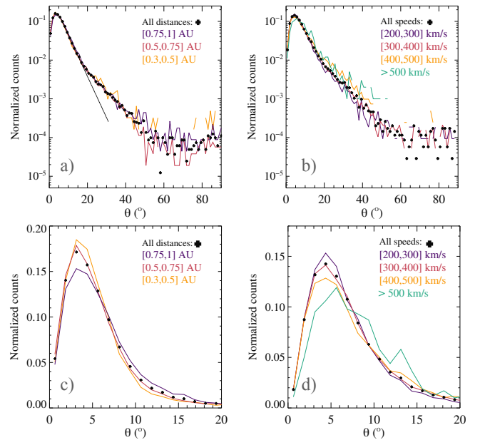
Fig. 3: Panel a) : Normalized histogram of the number of whistler waves as a function of the propagation angle for different heliocentric distances. Panel b) : Normalized histogram of the number of whistler waves as a function of the propagation angle for different solar wind speeds. Panel c) : Same as panel a) zoomed between 0 and 20°. Panel d) : Same as panel b) zoomed between 0 and 20°.
