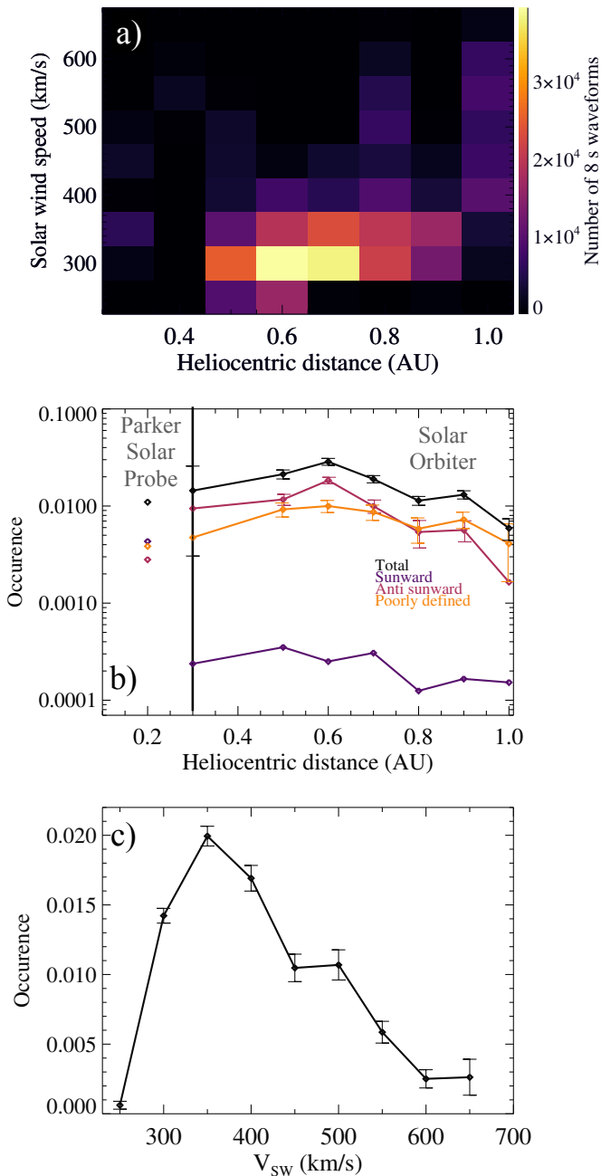
Fig. 2: Panel a) : Number of analyzed 8s-waveforms with Solar Orbiter as a function of heliocentric distance and solar wind speed. Panel b) : Whistler wave occurrence as a function of heliocentric distance for sunward, anti-sunward, and poorly defined propagation direction. When, due to low statistics, the 95% confidence intervals (calculated assuming a normal distribution) are of the order of magnitude of values, they are not shown. Panel c) : Occurrence as a function of the solar wind speed.
