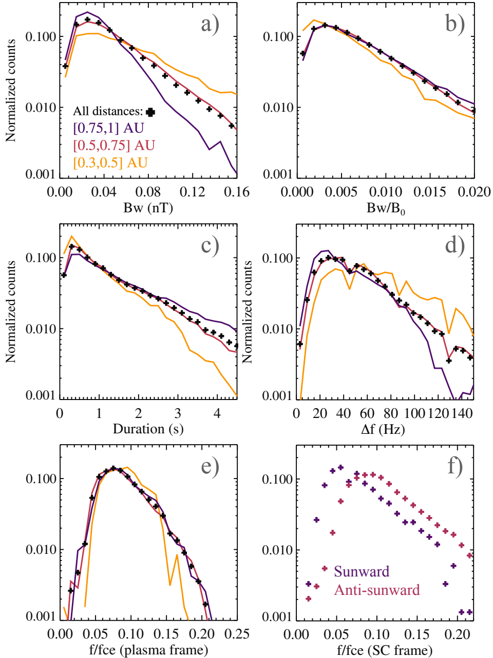
Fig. 5: Panels a) to e) : Normalized histograms for different wave parameters as a function of heliocentric distance. The wave parameters are as follows: Panel a) : Wave amplitude. Panel b) : Wave amplitude normalized by the the background magnetic field. Panel c) : Duration of the wave packets. Panel d) : Frequency width. Panel e) : Frequency in the plasma frame normalized by the local electron cyclotron frequency. Panel f) : Histogram of the frequency in the spacecraft frame normalized by the electron cyclotron frequency for sunward (in purple) and anti-sunward whistler waves (in pink).
