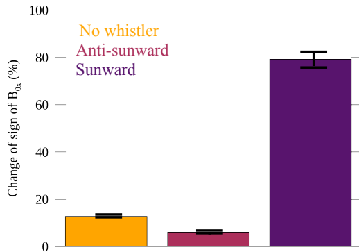
Fig. 7: Percentage of cases in which the sign of the radial component of the background magnetic field during the measurement is not the median sign of this component over a 24-hour period centered on the measurement. To produce this figure, we use only Solar Orbiter data.
