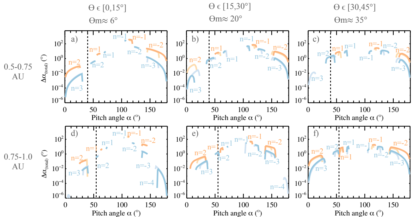
Fig. 9: Integrated diffusion coefficients at two heliocentric distance and three propagation angle \theta bins. Legends and notations are similar to Figure 8.
