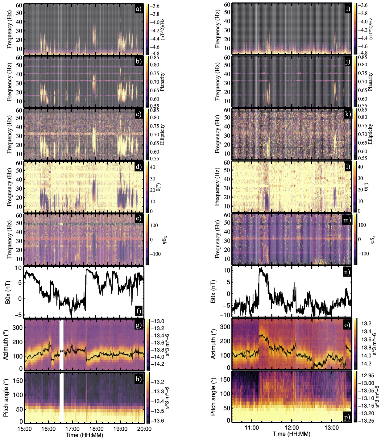
Fig. 6: Observations of whistler waves activities with Solar Orbiter on 2021/08/15 on the left and 2021/10/08 on the right. Panels a) to e) and i) to m) : Spectrograms of several wave parameters calculated from CWF with: Panels a) and i) : Power spectral density. Panels b) and j) : Planarity. Panels c) and k) : Ellipticity. Panels d) and l) : Propagation angle. Panels e) and m) : \varphi S_x . Panels f) and n) : X components of the background magnetic field. Panels g) and o) : Velocity distribution functions (summed over energies between 100 and 1000 eV and over all elevations) as a function of time and azimuth angle of EAS 1 with the azimuth of the background magnetic field in black (in the EAS 1 reference frame). Panels h) and p) : Pitch angle distribution (summed over energies between 100 and 1000 eV) using EAS 1 and EAS 2 data.
