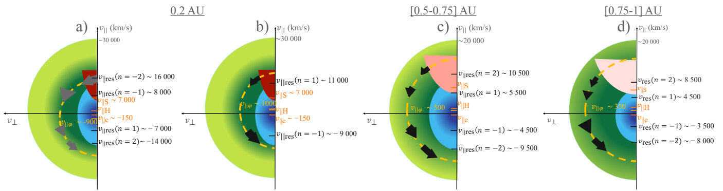
Fig. 11: Scheme of the evolution of the e-VDF in the (v_{\perp}, v_{\parallel}) plane and its interaction with whistler waves as a function of heliocentric distance. Panel a) represents the effect of counter-streaming whistler waves at 0.2 AU. Panels b), c), d) show the effect of Strahl-aligned whistler waves between 0.2 and 1 AU. The blue circles represent the core electrons, the green circles the halo electrons, and the red/pink beams the Strahl electrons. The intensity of the color represents the population's relative density. The resonance velocities ( v_{\text{res}||} ) for n = \pm 1 and n = \pm 2 , the drift velocities of the core, halo and Strahl (noted v_{c||}, v_{H||}, v_{S||} , respectively), and the parallel phase velocities v_{\phi||} of the waves are indicated along the v_{\parallel} axis. The resonance velocities with n = \pm 3 are not represented for clarity. One of the single-wave characteristics (centered around v_{\phi||} ) is represented by an orange dotted line. The path of the diffusing electrons is indicated by the arrows. This diffusion takes place around parallel resonance speeds. The role of the diffusing electrons in the amplification (resp., damping) of the waves is represented by black (resp., grey) arrows.
